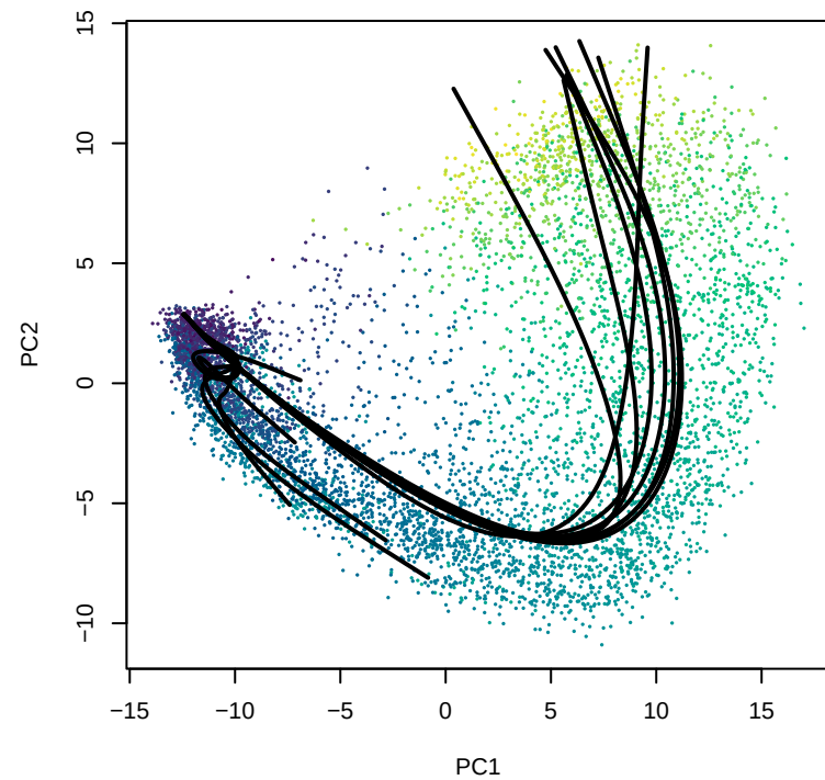
Slingshot average pseudotime
