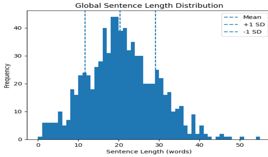
global_sentence_length_distribution.png
