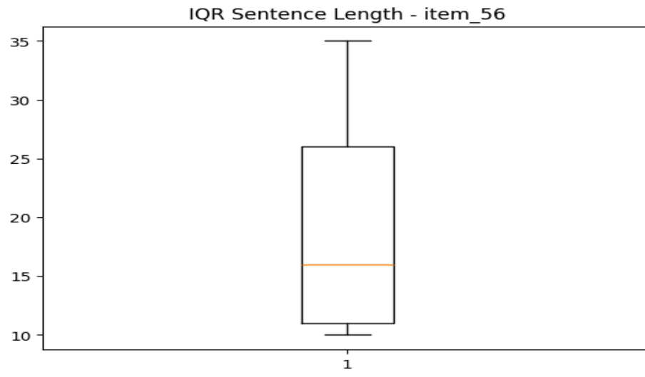
sentence_IQR_item_56.png
