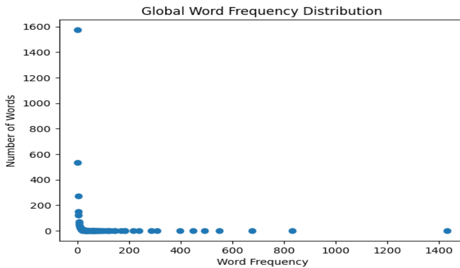
global_word_freq_distribution.png
