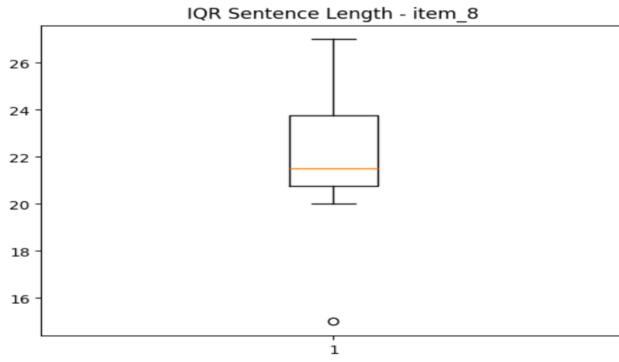
sentence_IQR_item_8.png
