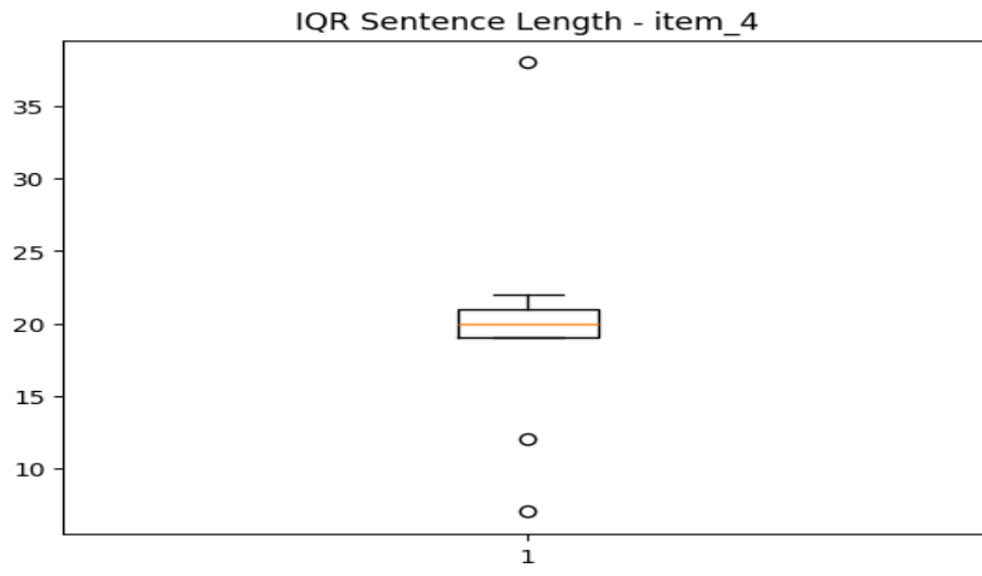
sentence_IQR_item_4.png
