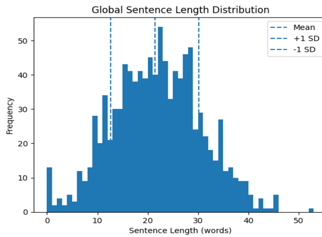
global_sentence_length_distribution.png
