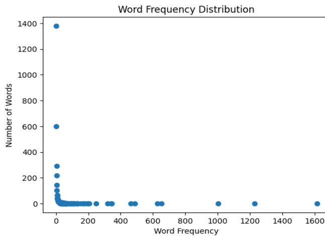
global_word_freq_distribution.png
