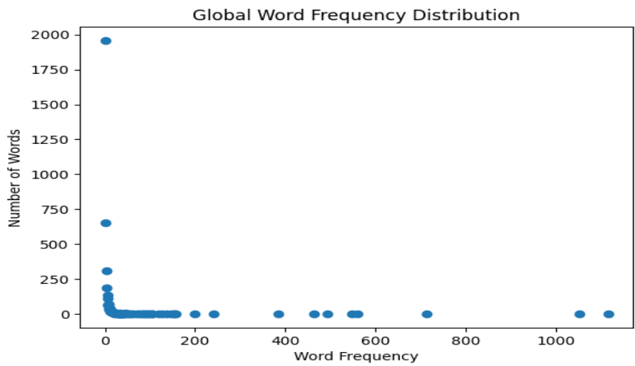
global_word_freq_distribution.png
