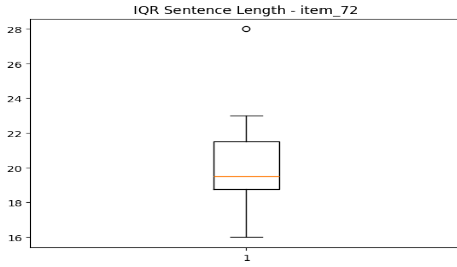
sentence_IQR_item_72.png
