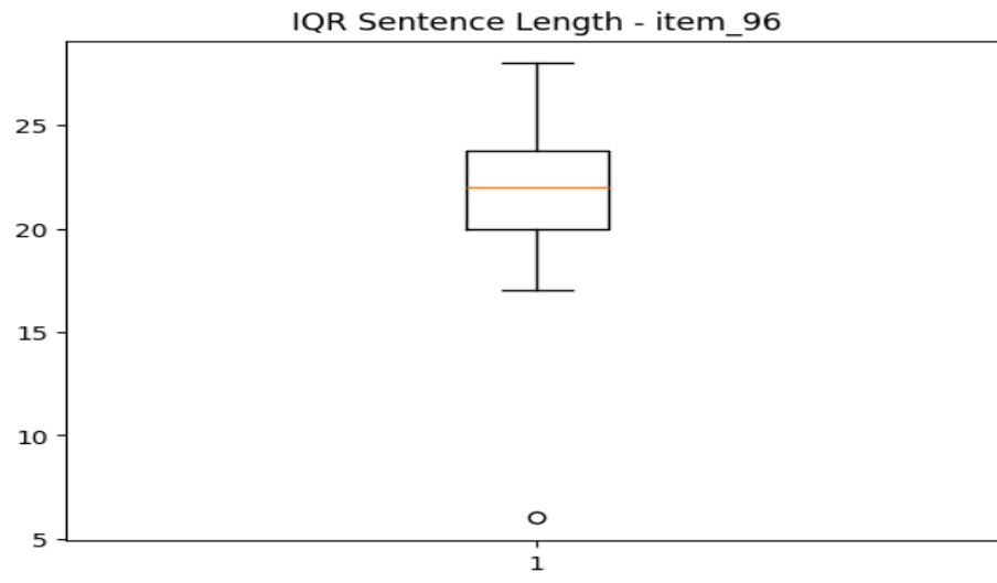
sentence_IQR_item_96.png
