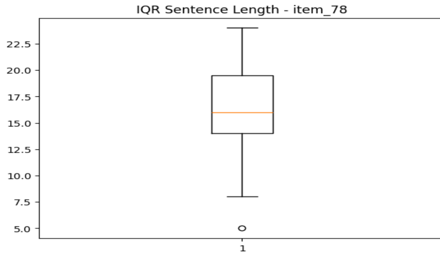
sentence_IQR_item_78.png
