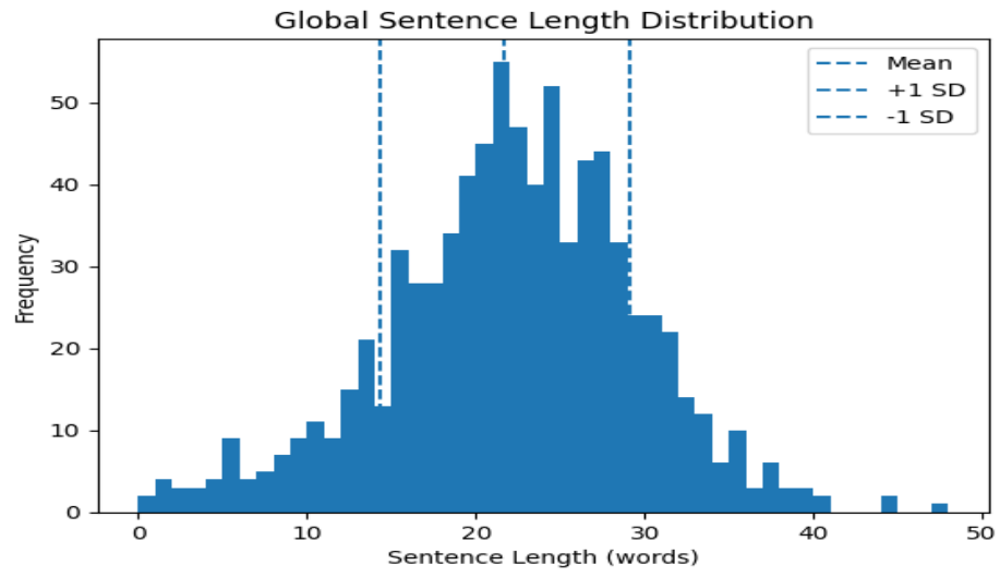
global_sentence_length_distribution.png
