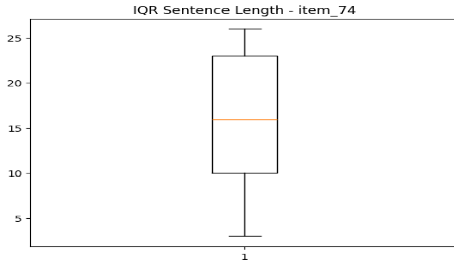
sentence_IQR_item_74.png
