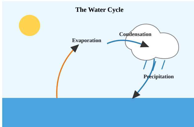
Figure 1: The water cycle
