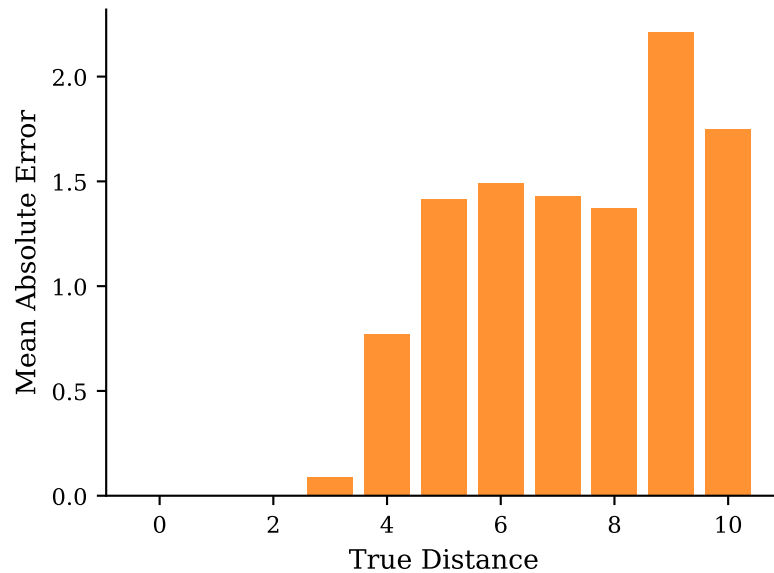
Heuristic MAE by Distance
