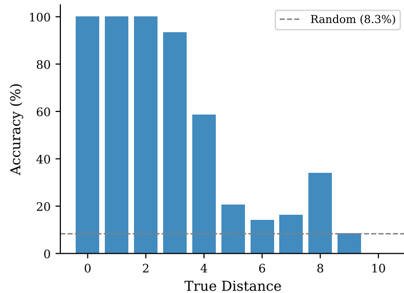
Per-Distance Accuracy
