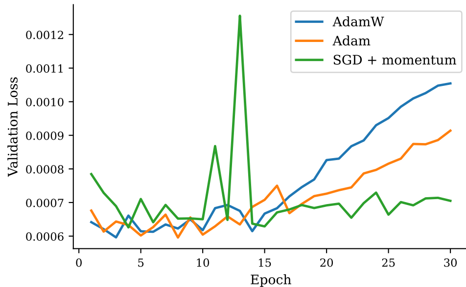
Loss by Optimizer
