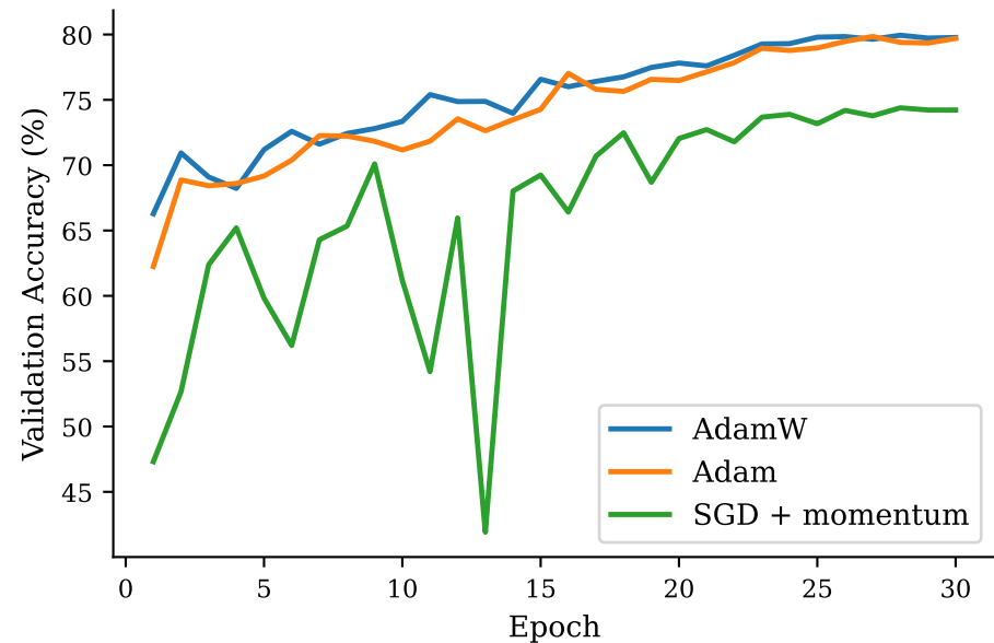
Accuracy by Optimizer
