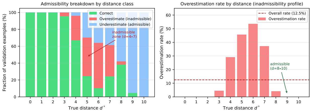
Figure 6: Per-distance admissibility breakdown (left) and overestimation rate (right) for the AdamW + cosine model. Left: stacked bars show the fraction of validation examples at each true distance d^* that are correctly predicted, overestimated ( \hat{d} > d^* , inadmissible), or underestimated ( \hat{d} < d^* , admissible). Right: the overestimation rate peaks at d = 5-6 ( > 50\% ) and drops to zero for d = 8-10 ; the dashed line marks the overall rate of 12.5%. Inadmissibility is concentrated in the mid-range distance classes where classification is most uncertain.
