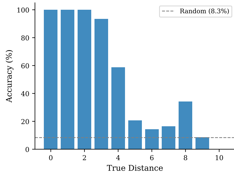
Per-Distance Accuracy
