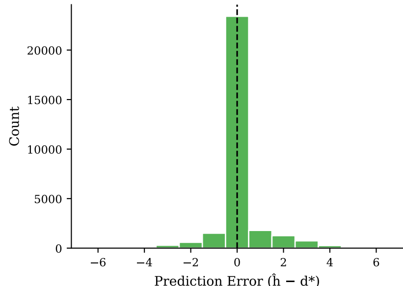
Error Distribution
