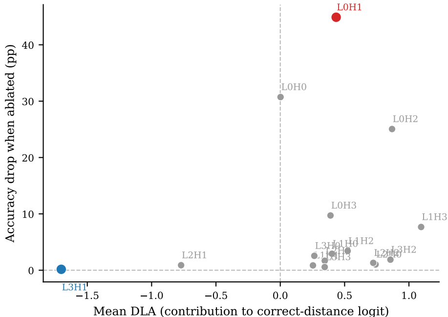
Per-head DLA vs. ablation sensitivity (baseline 76.2%)
