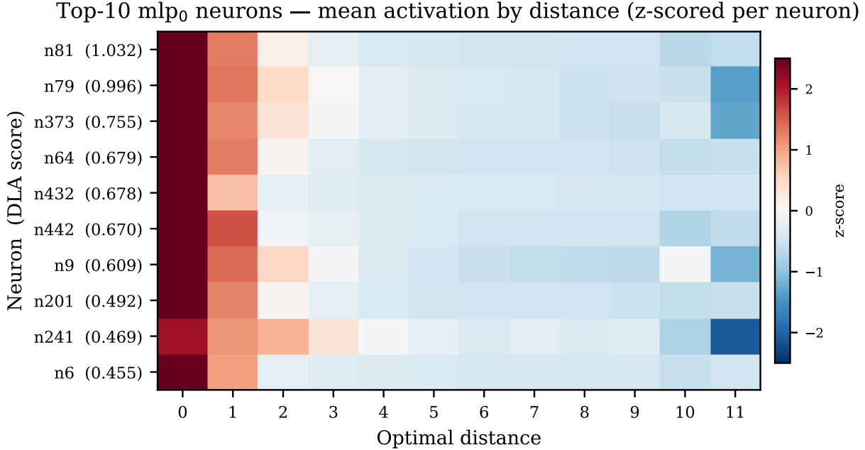
Figure 2: Mean activation of the top-10 \text{mlp}_0 neurons by optimal distance, z-scored per neuron. Red = high activation; blue = low. All neurons are monotonically tuned to distance, confirming that \text{mlp}_0 computes distance rather than geometric features such as face-solved or corner-oriented status.
