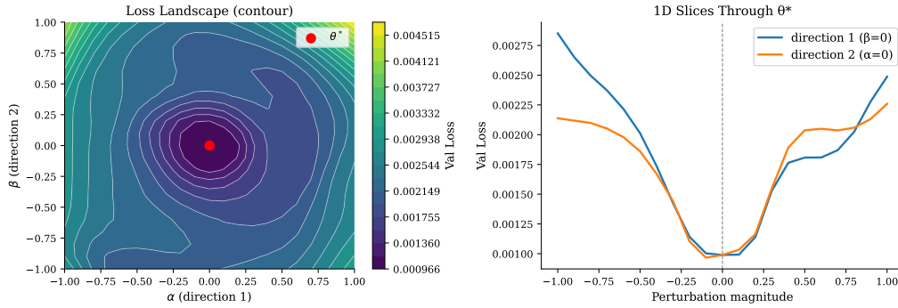
Figure 5: Filter-normalized loss landscape around \theta^* (left: contour plot; right: 1D slices through the solution). The center loss is \mathcal{L}(\theta^*) = 0.0010 ; the maximum across the 21 \times 21 grid is 0.0047—only 4.76\times the center value—despite perturbation magnitudes as large as the filter norms themselves. Both 1D slices are smooth and bowl-shaped, indicating a wide, flat minimum.
