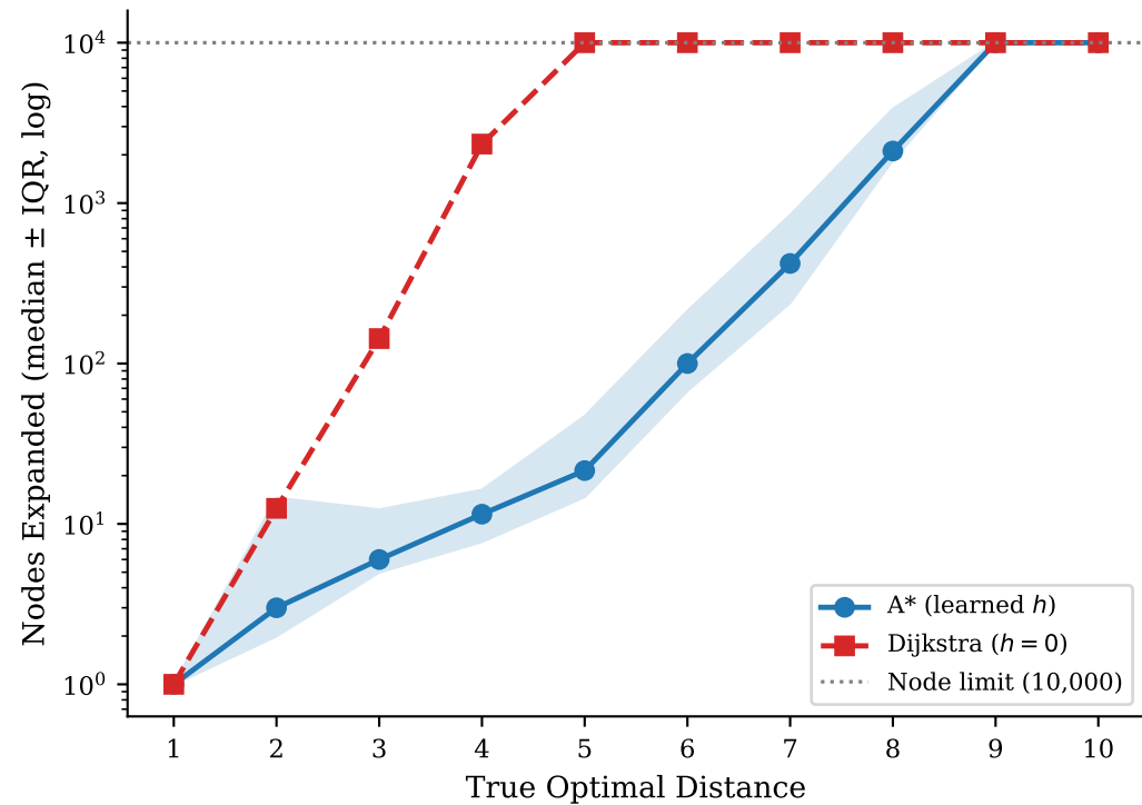
Search Efficiency
