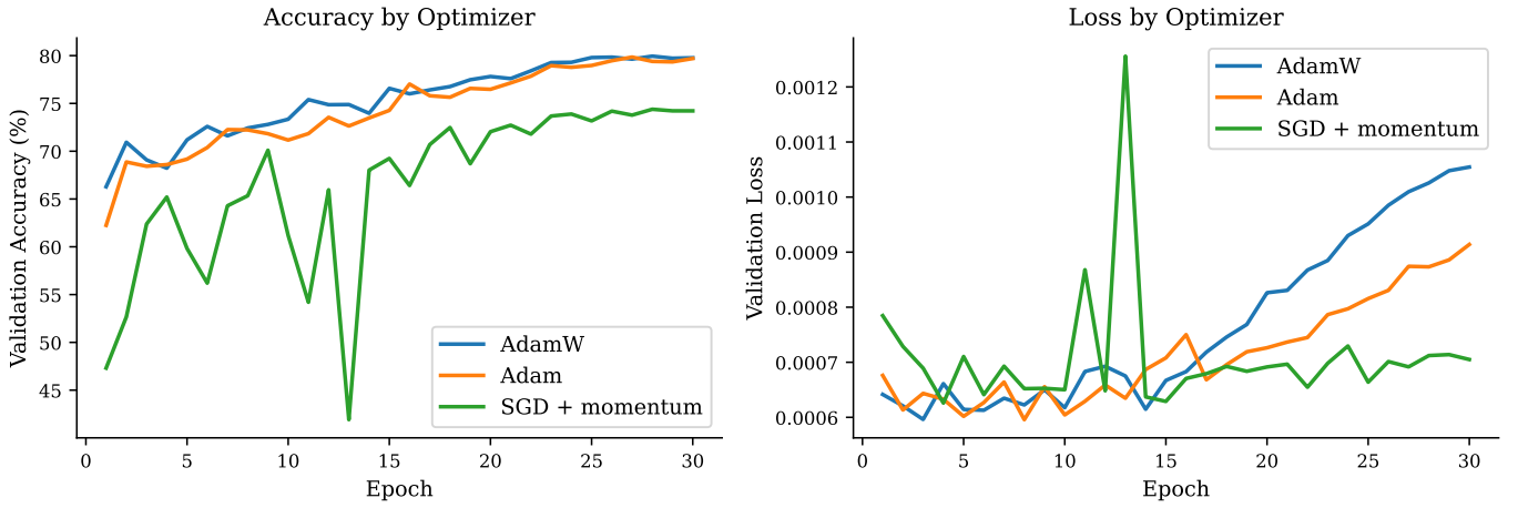
Fig. 1. Validation accuracy (left) and loss (right) over 30 training epochs for AdamW, Adam, and SGD with momentum, all under cosine annealing. AdamW and Adam converge to nearly identical final accuracy (79.9% and 79.8%), while SGD trails by 5.5 pp (74.4%).
