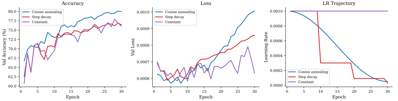
Fig. 2. Validation accuracy (left), loss (center), and learning rate trajectory (right) for three schedules under AdamW. Cosine annealing (80.1%) outperforms step decay (76.9%) and constant (77.9%).
