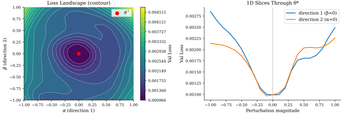
Fig. 6. Filter-normalized loss landscape around \theta^* (left: contour plot; right: 1D slices through the solution). The center loss is \mathcal{L}(\theta^*) = 0.0010 ; the maximum across the 21 \times 21 grid is 0.0047—only 4.76\times the center value—despite perturbation magnitudes as large as the filter norms themselves. Both 1D slices are smooth and bowl-shaped, indicating a wide, flat minimum.
