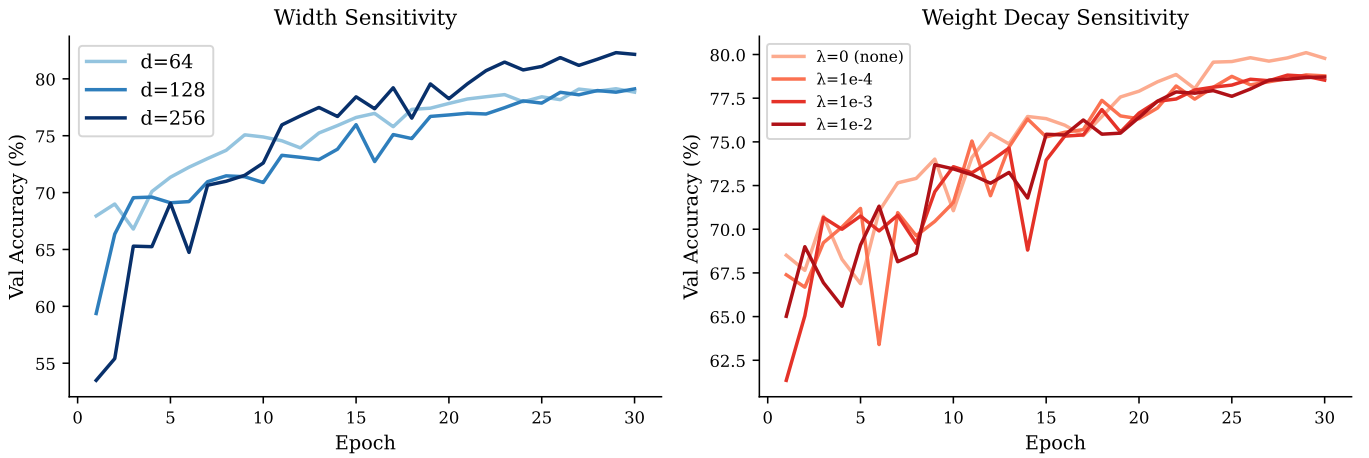
Fig. 3. Convergence curves for the model width sweep (left) and weight decay sweep (right). Width d_{\text{model}} = 256 outperforms 128 and 64 by 3.2 pp; all weight decay values produce similar final accuracy, with no decay ( \lambda = 0 ) performing best.
