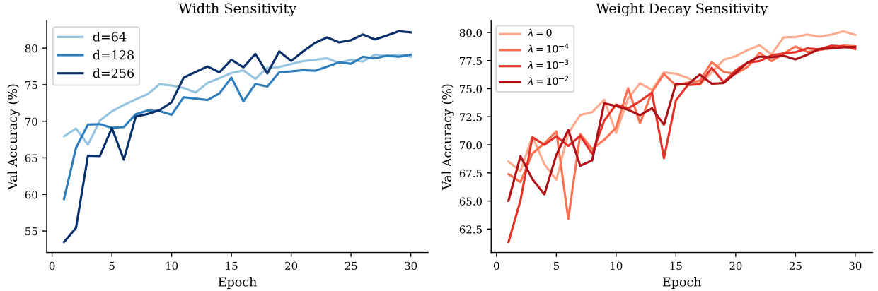
Figure 4: Convergence curves for the model width sweep (left) and weight decay sweep (right). Width d_{\text{model}} = 256 outperforms 128 and 64 by 3.2 pp; all weight decay values produce similar final accuracy, with no decay ( \lambda = 0 ) performing best.
