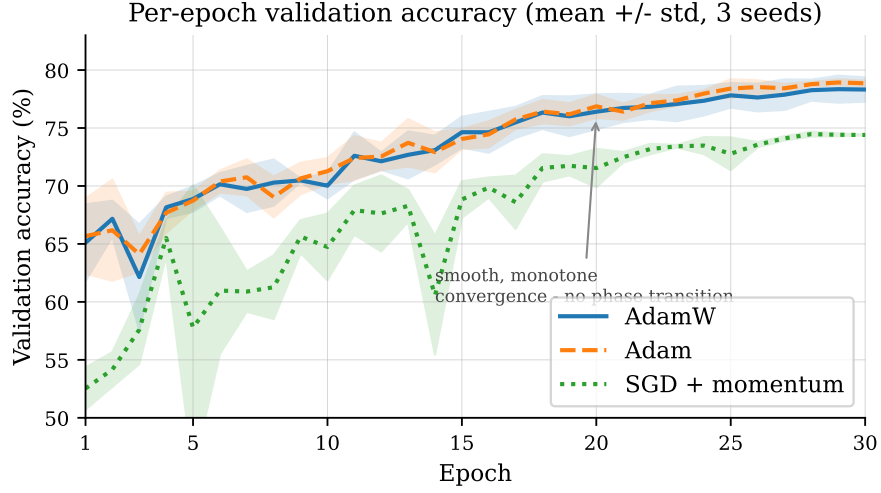
Figure 3: Per-epoch validation accuracy (mean \pm std shading over 3 seeds) for AdamW, Adam, and SGD with momentum under cosine annealing. All three optimizers converge smoothly and approximately monotonically—no sudden generalization jump or grokking-style phase transition is observed. SGD lags throughout but narrows the gap in later epochs as the schedule reduces the learning rate.
