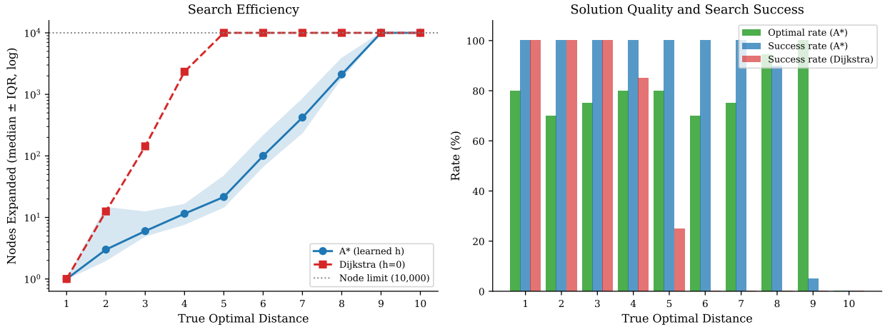
Figure 7: Left: median nodes expanded (log scale, shaded IQR for A*) vs. true optimal distance; the dotted line marks the 10,000-node limit. Right: A* solution optimality rate (green), A* search success rate (blue), and Dijkstra success rate (red). Dijkstra begins to fail at d = 4 and collapses at d \geq 6 ; A* achieves 100% success through d = 7 and finds optimal solutions 70–80% of the time for d \leq 7 .
