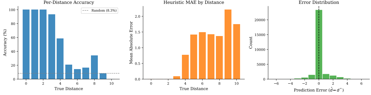
Figure 5: Left: per-distance accuracy (dashed line = random baseline 8.3%). Center: mean absolute error by true distance. Right: distribution of prediction errors \hat{d} - d^* ; negative values are underestimates (admissible), positive values are overestimates (inadmissible). The distribution is centered slightly below zero, reflecting a weak tendency toward underestimation.
