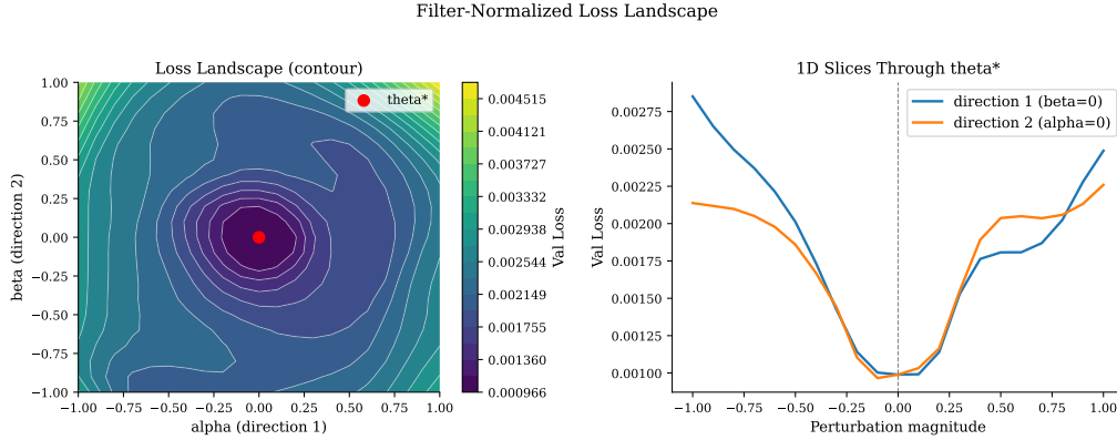
Figure 8: Filter-normalized loss landscape around \theta^* (left: contour plot; right: 1D slices through the solution). The center loss is \mathcal{L}(\theta^*) = 0.0010 ; the maximum across the 21 \times 21 grid is 0.0047—only 4.76\times the center value—despite perturbation magnitudes as large as the filter norms themselves. Both 1D slices are smooth and bowl-shaped, indicating a wide, flat minimum.
