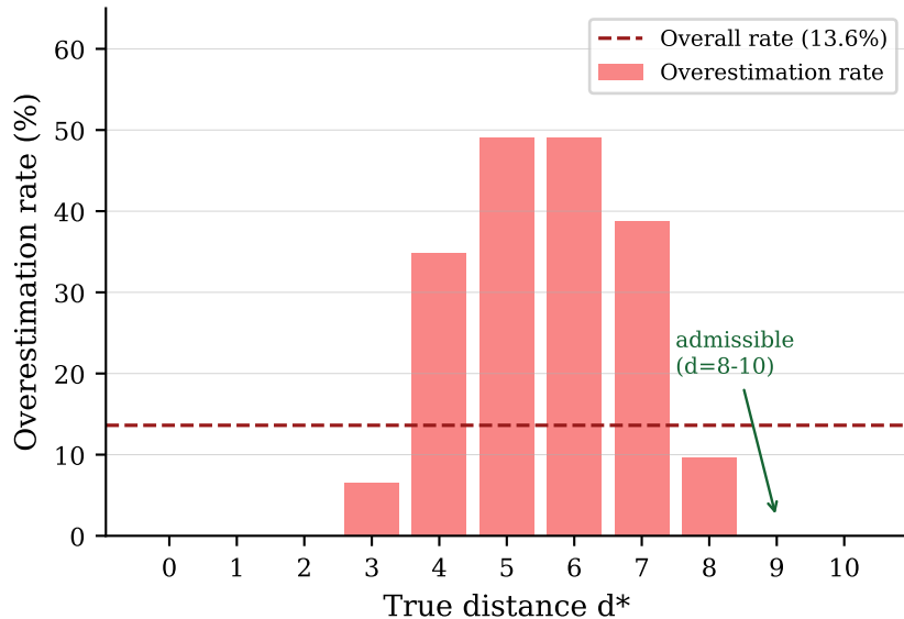
Overestimation rate by distance (inadmissibility profile)
