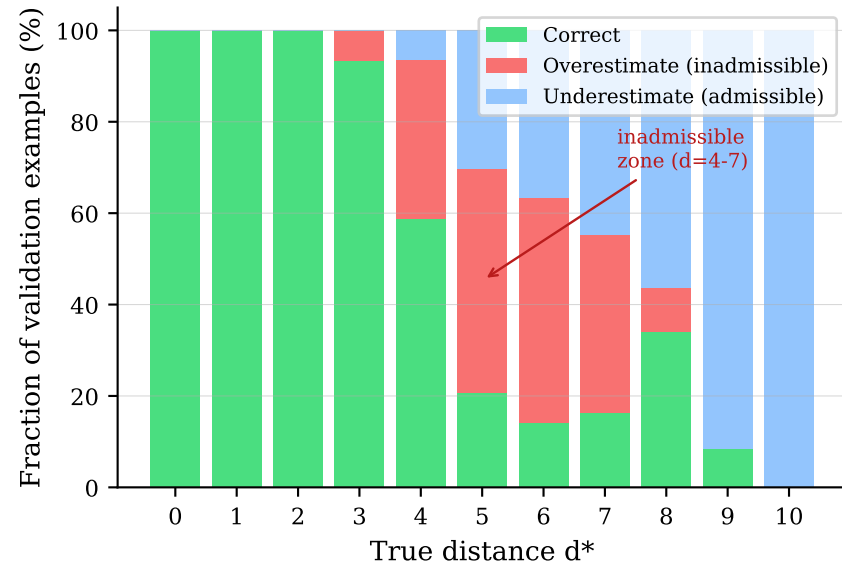
Admissibility breakdown by distance class
