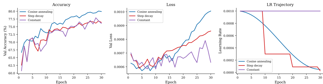
Figure 2: Validation accuracy (left), loss (center), and learning rate trajectory (right) for three schedules under AdamW. Cosine annealing Mean \pm std over 3 seeds: cosine 78.3 \pm 1.0\% , step 77.5 \pm 1.3\% , constant 77.2 \pm 1.0\% .
