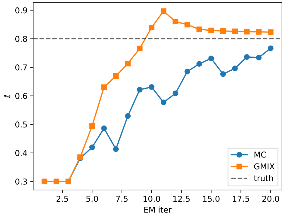
Lengthscale path ( T=20000 , \ell_{\text{true}}=0.8 )
