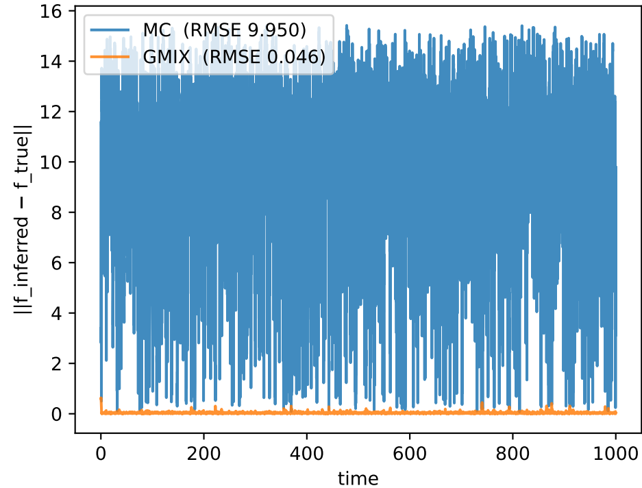
Drift error along true trajectory
