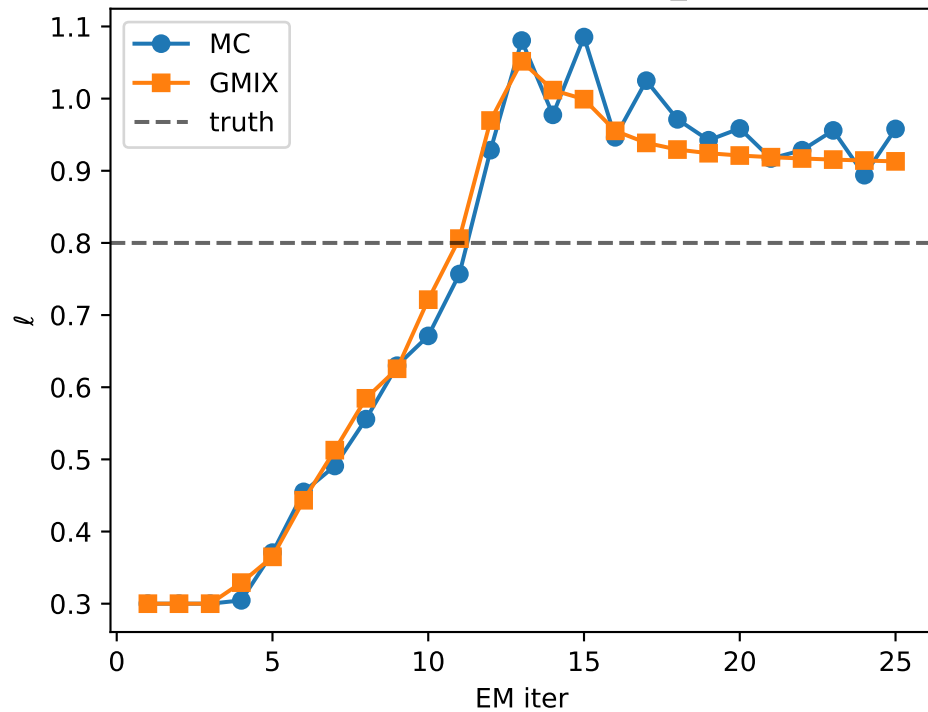
Lengthscale path ( T=2000 , \ell_{\text{true}}=0.8 )
