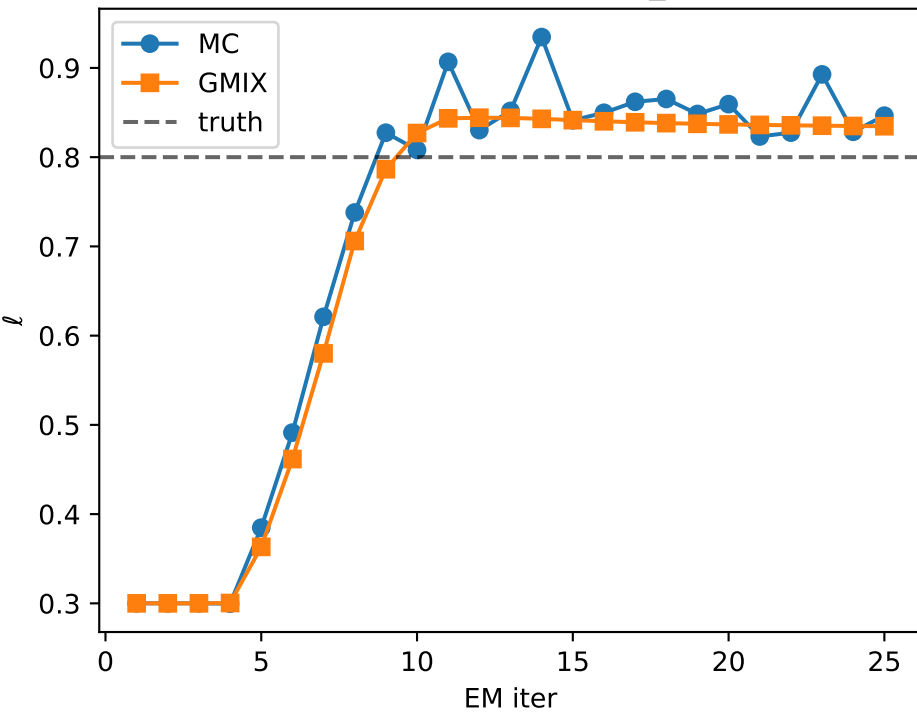
Lengthscale path ( T=500 , \ell_{\text{true}}=0.8 )
