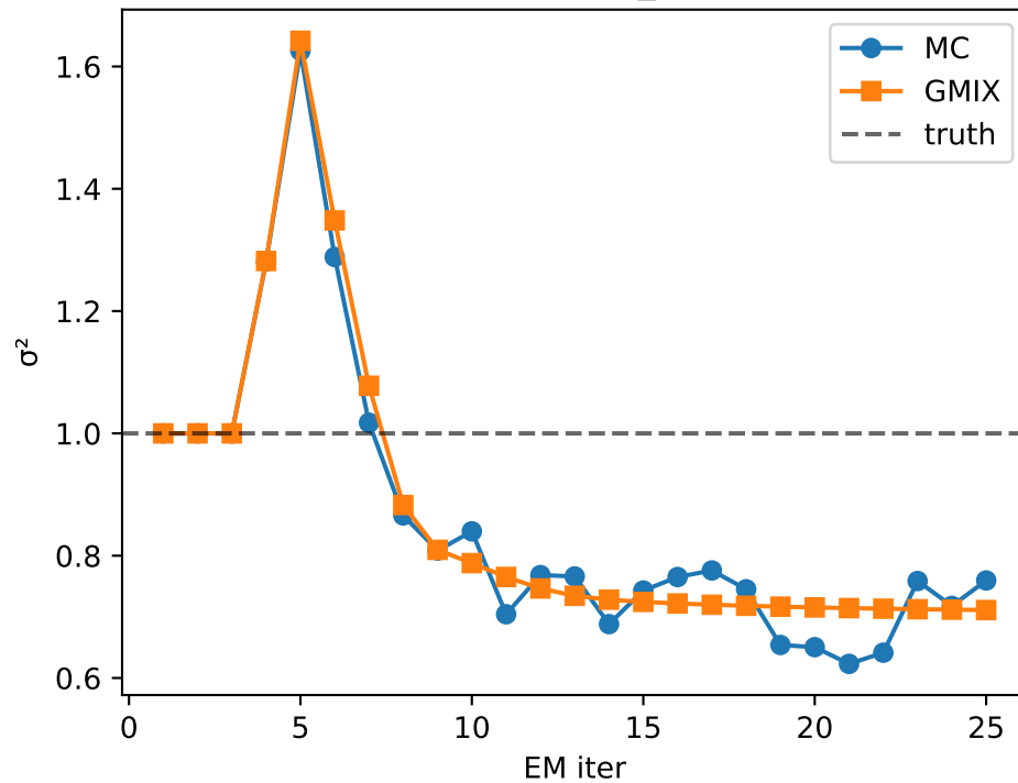
Variance path ( \sigma^2_{\text{true}}=1.0 )
