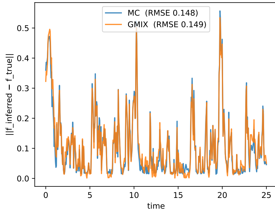
Drift error along true trajectory
