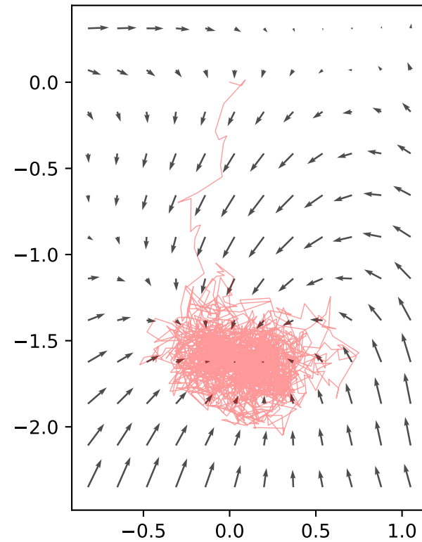
truth
