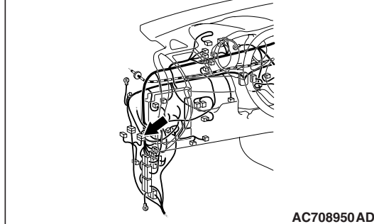
Connector: C-45
