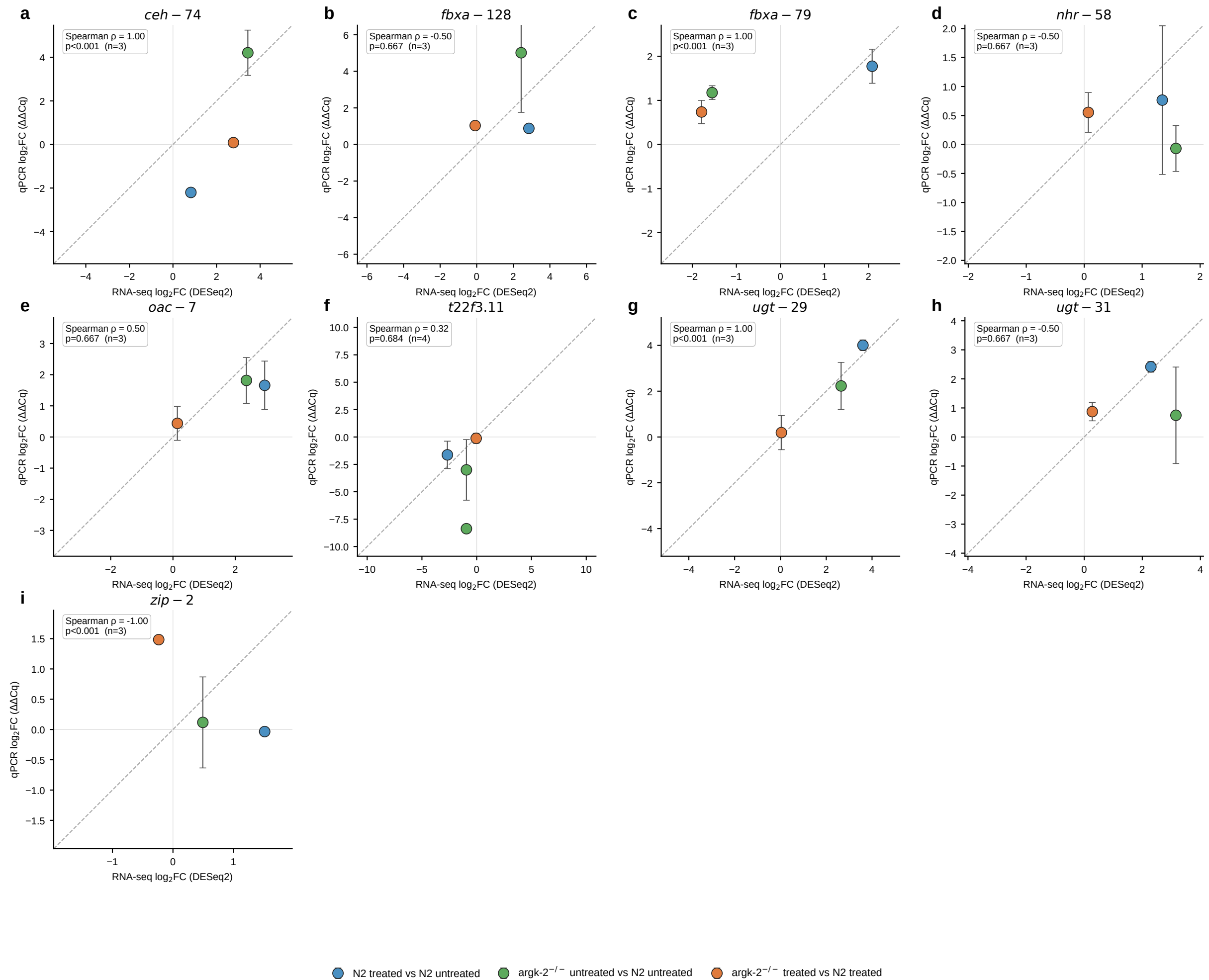
Supplementary Figure — Per-gene qPCR vs RNA-seq validation
