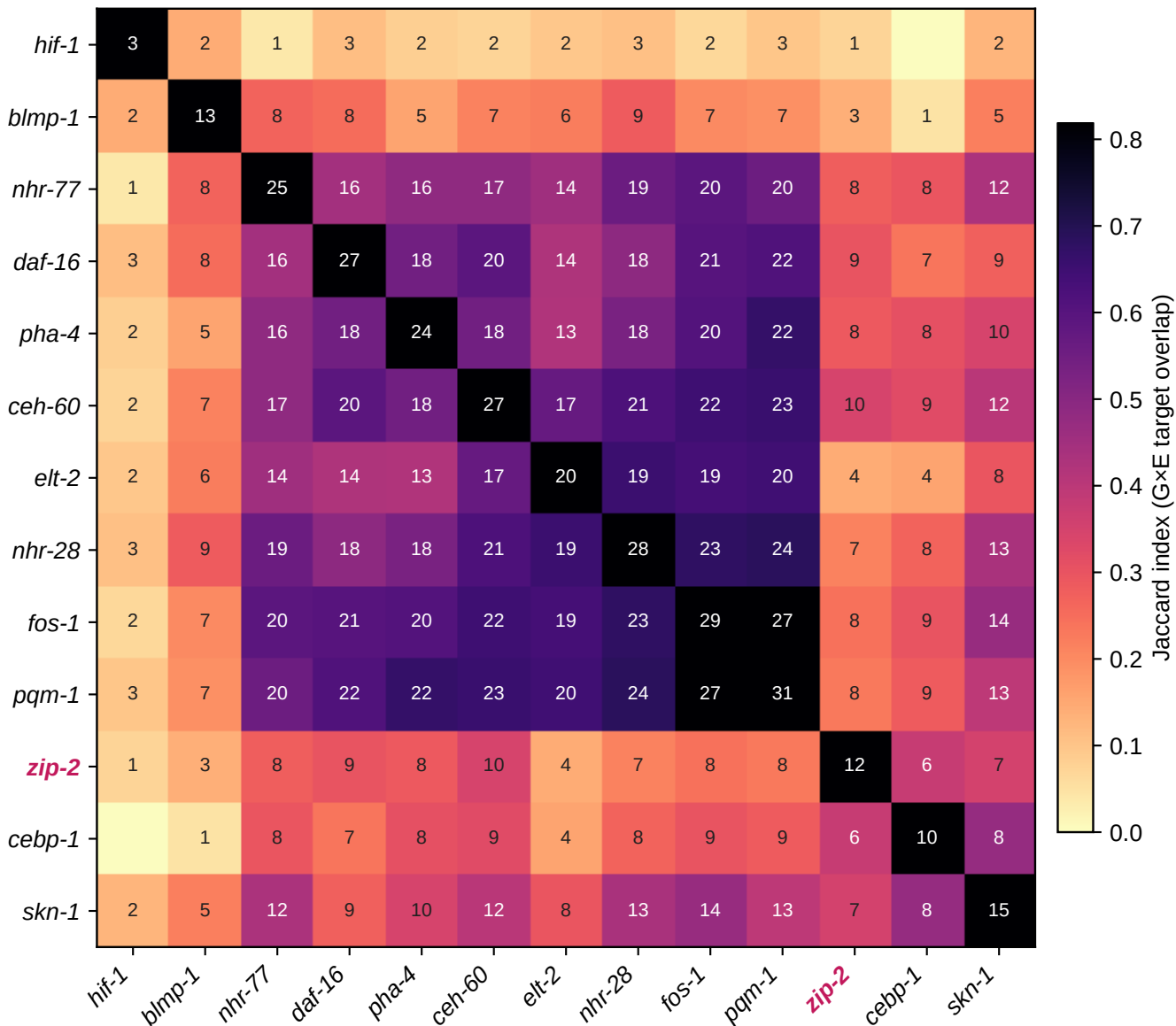
Hub-TF co-regulation of G×E genes (cells annotated with # shared G×E targets)
