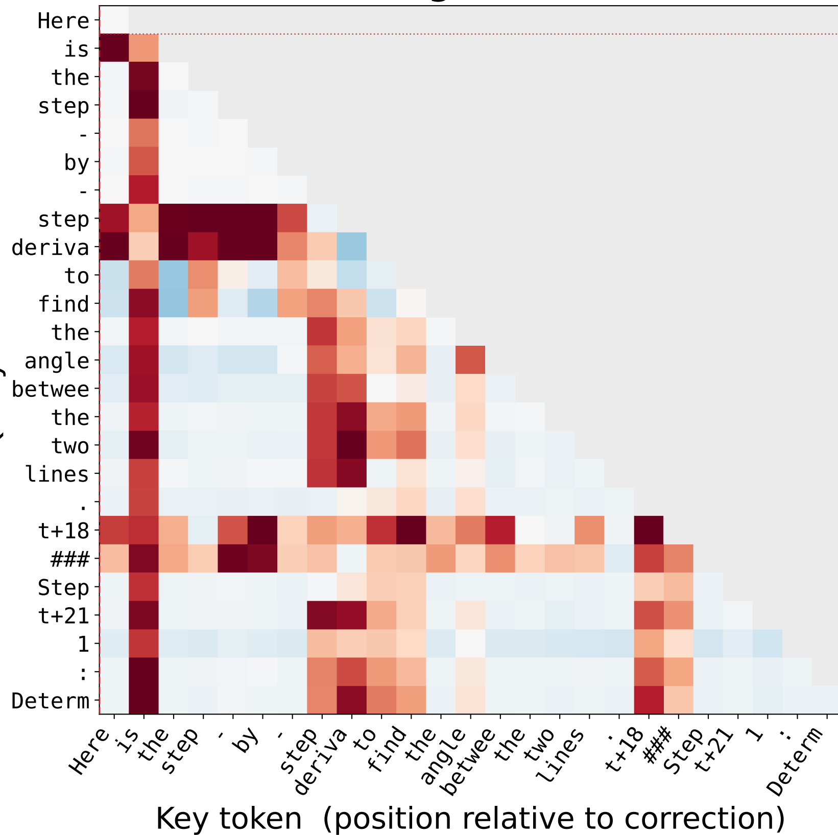
(a) Problem 1: angle between two lines
