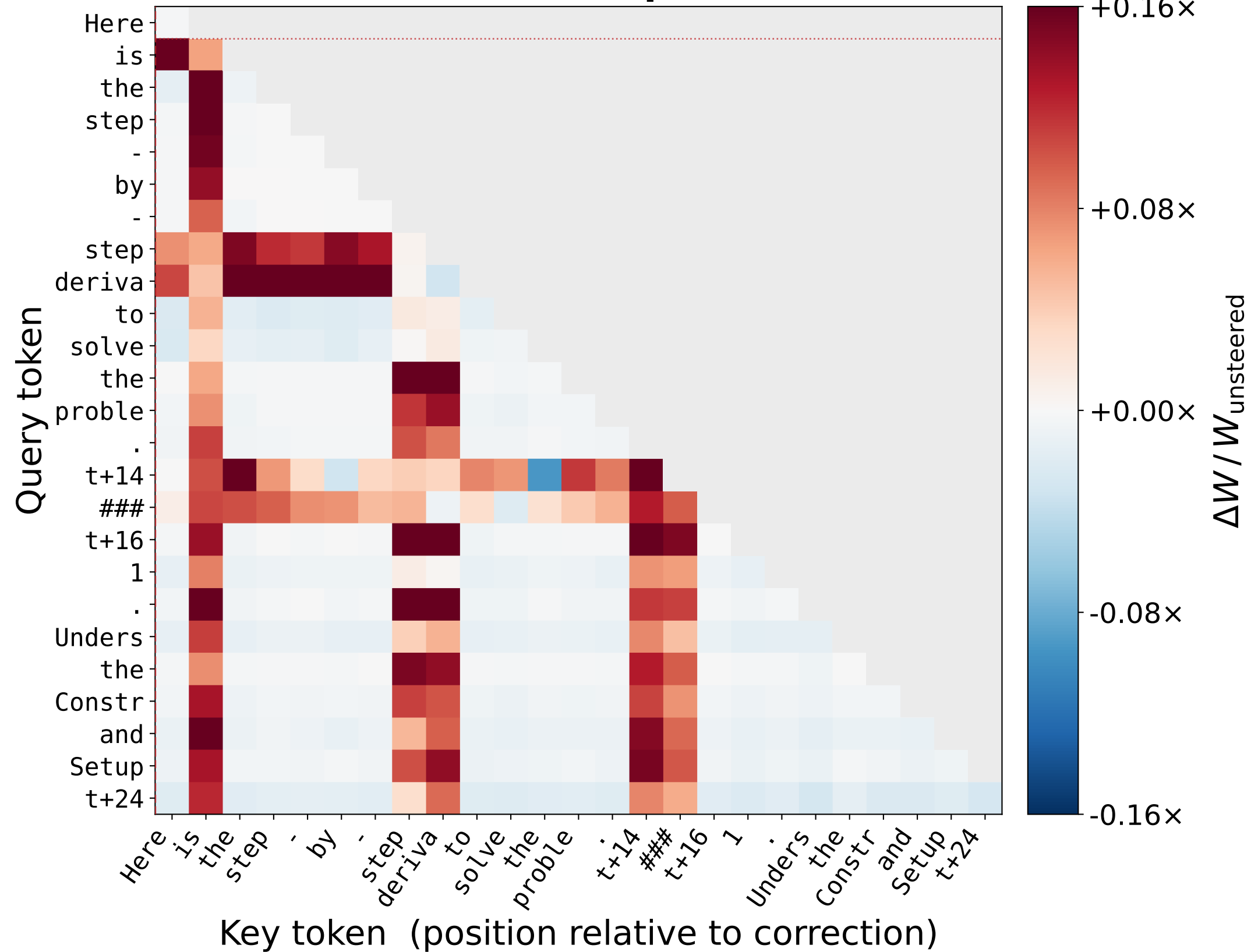
(b) Problem 2: complex rotation
