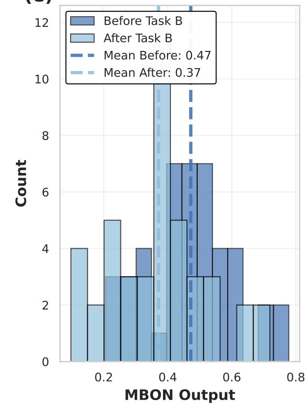
(e) E. MBON Population Drift ( \Delta=0.101 )
