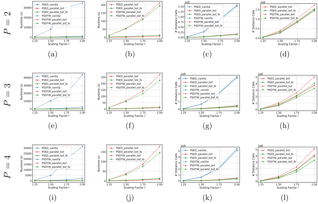
Figure 3.11: Comparing runtime and the number of distance calls for the methods with different P and l on the GunPoint dataset.
