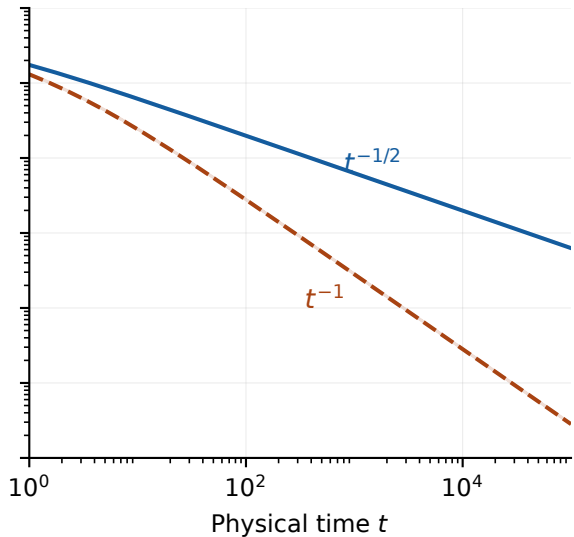
\mu = 1/2 : deformed law
