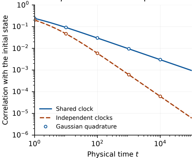
\mu = 1 : Gaussian endpoint
