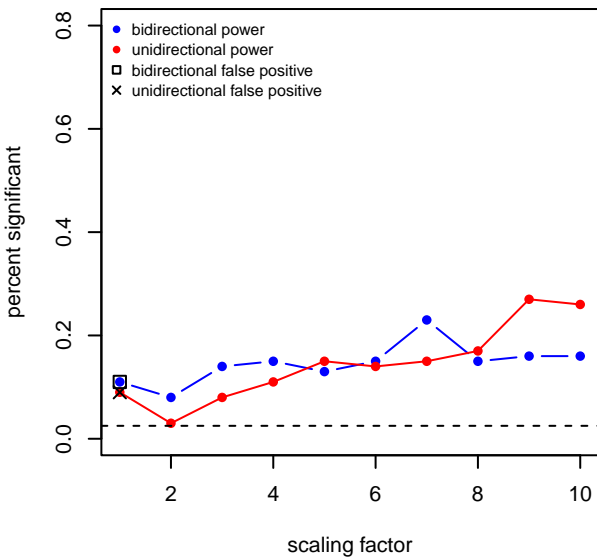
25 taxa
