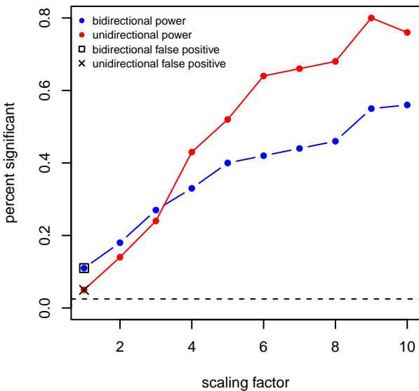
100 taxa
