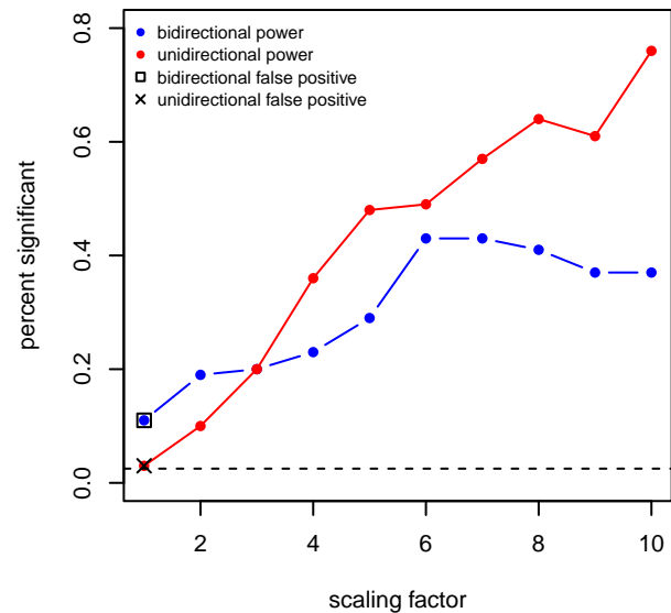
75 taxa
