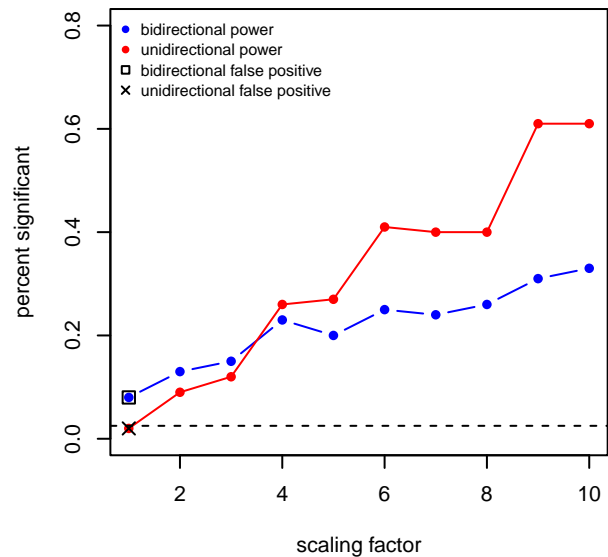
50 taxa
