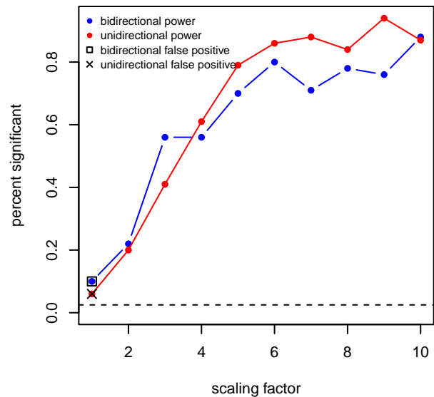
200 taxa
