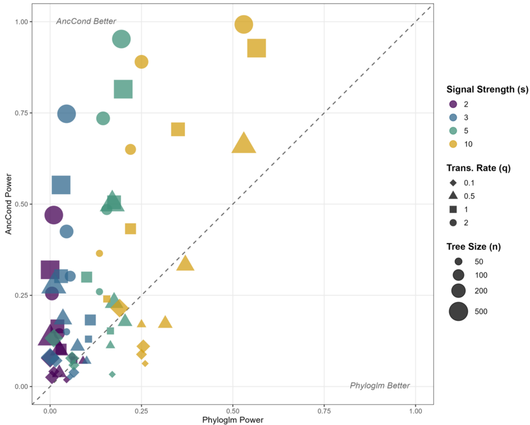
Head-to-Head Power Comparison
