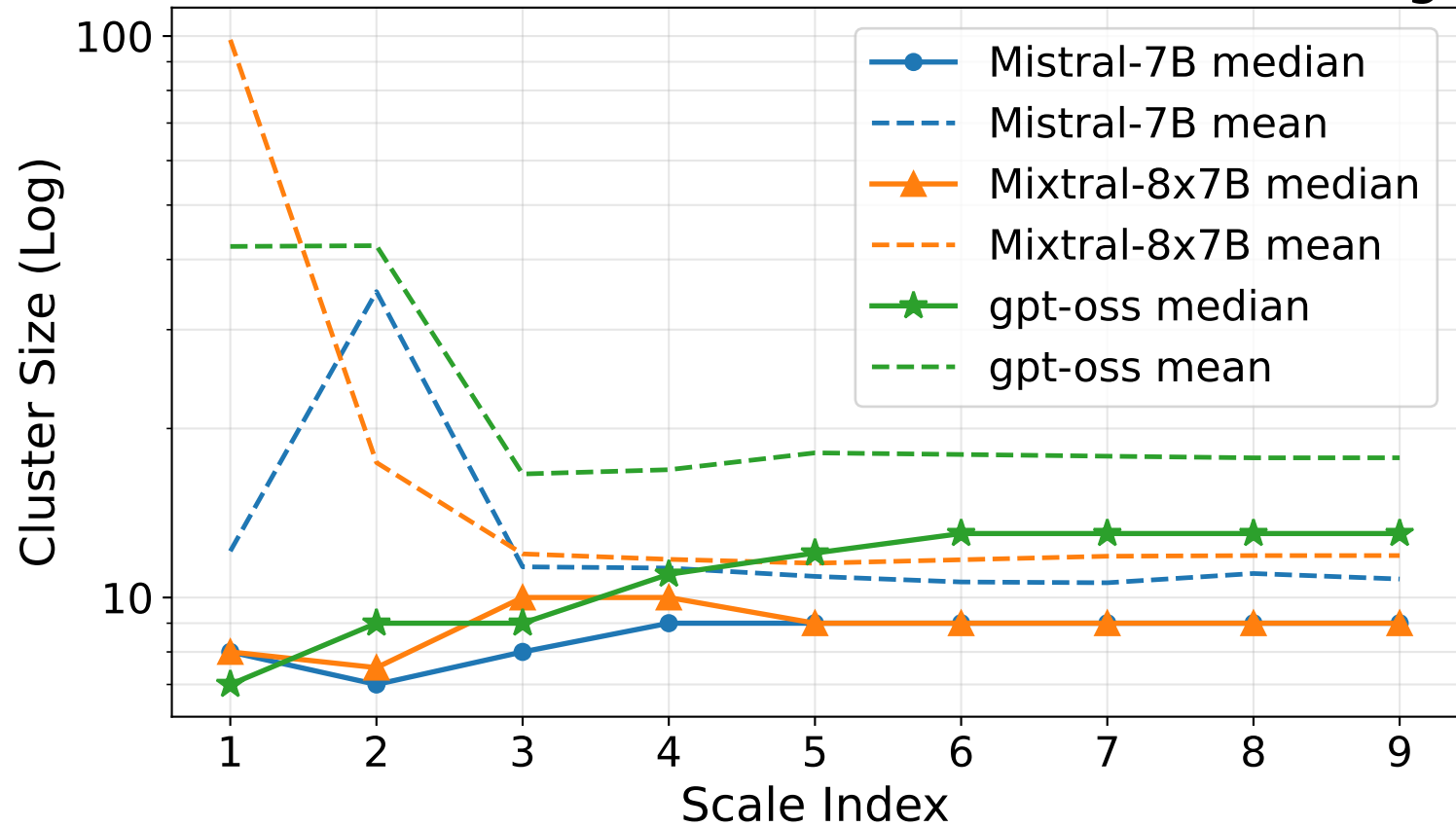
Full-PCA Cluster Size: Mean and Median (Log)
