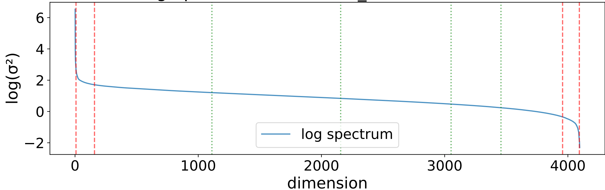
Log Spectrum of mistralai_Mixtral-8x7B-v0.1
