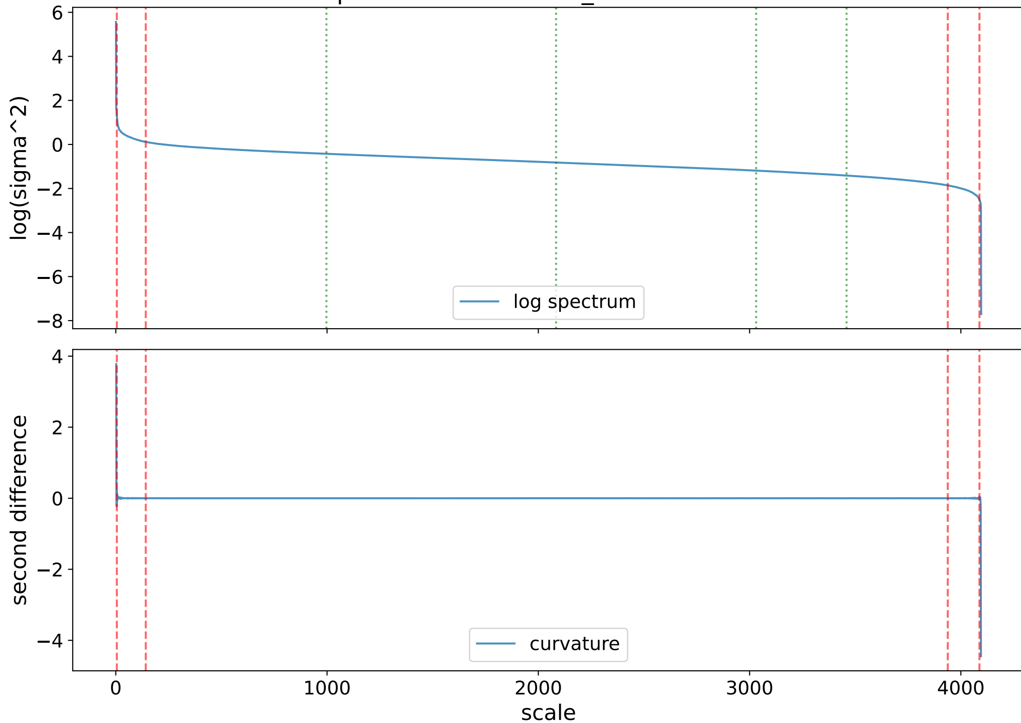
Spectrum of mistralai_Mistral-7B-v0.1
