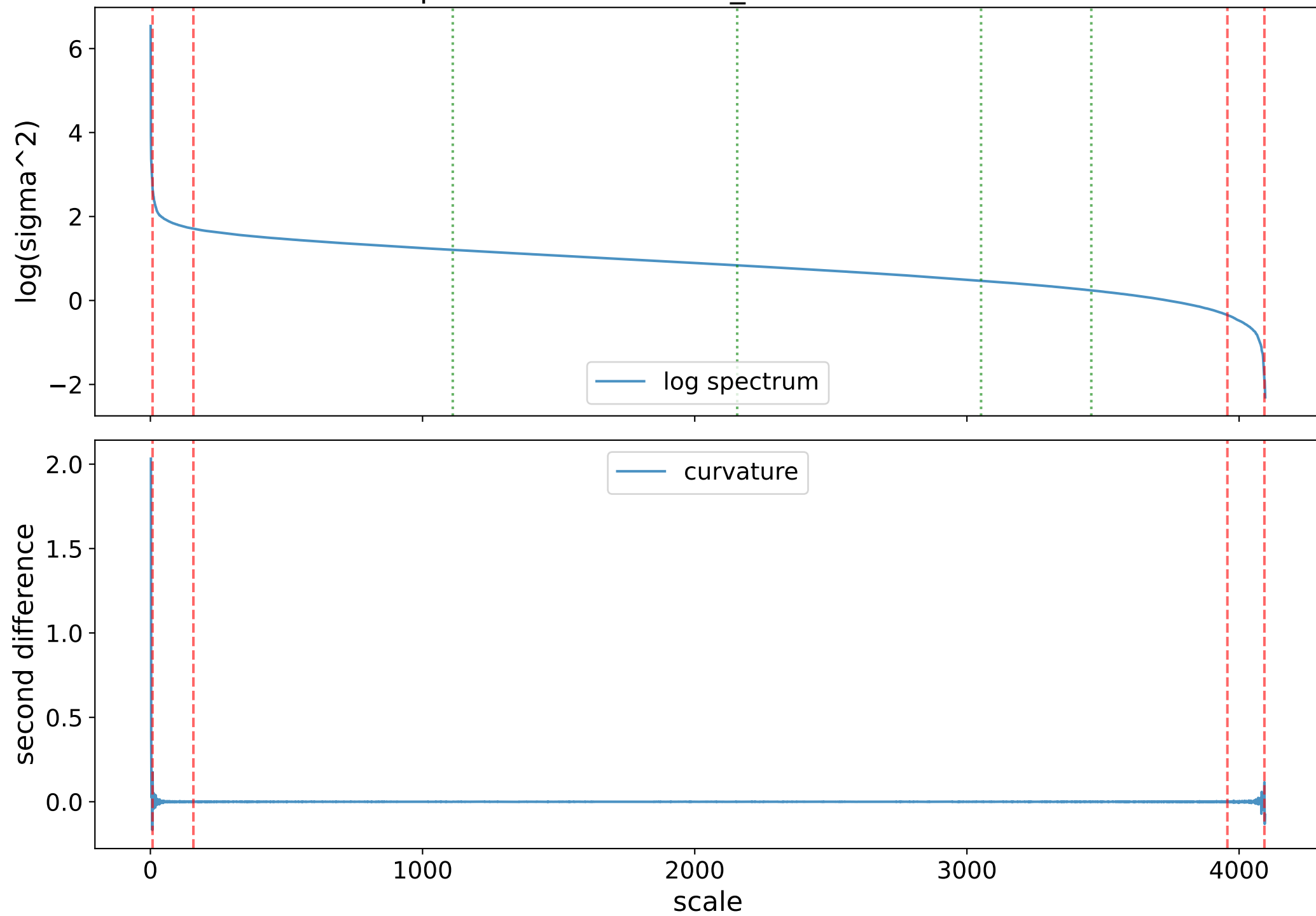
Spectrum of mistralai_Mixtral-8x7B-v0.1
