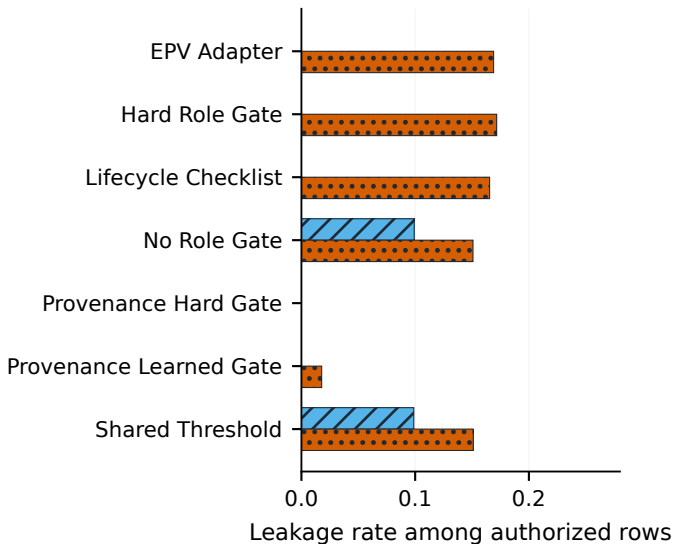
Role checks miss indirect laundering
