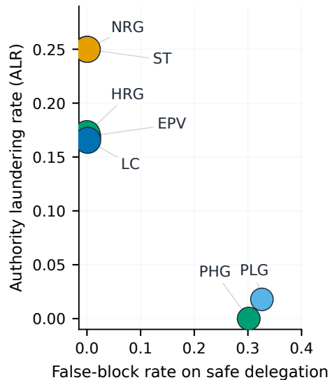
Delegation-integrity trade-off
