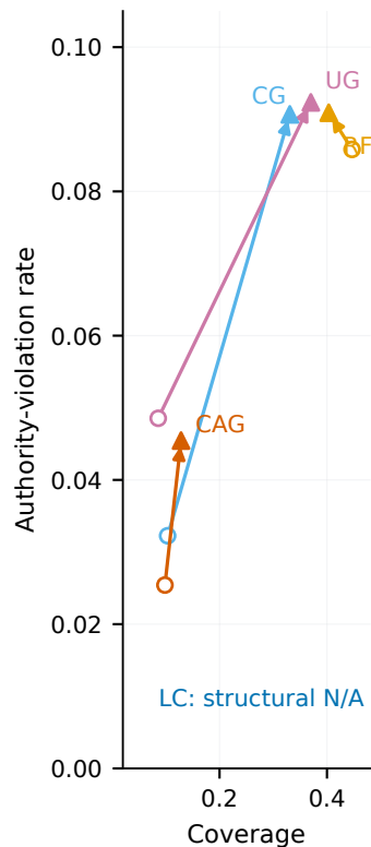
(c) Development-only recalibration
