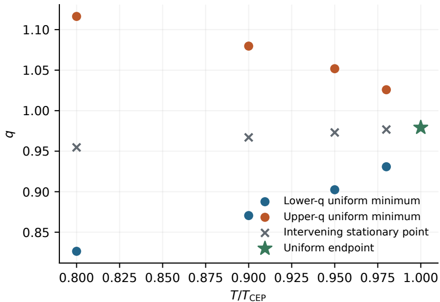
(a) Local uniform branch coalescence
