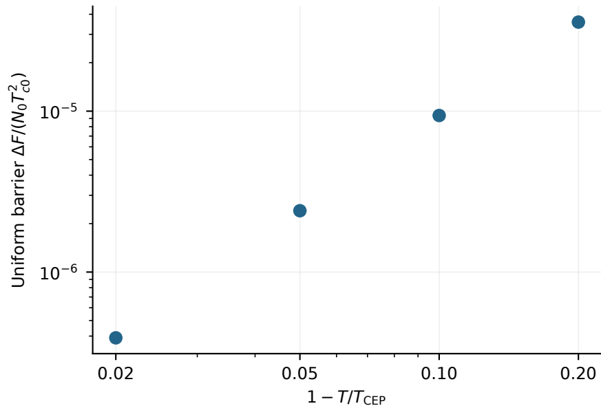
(b) Measured coexistence barriers
