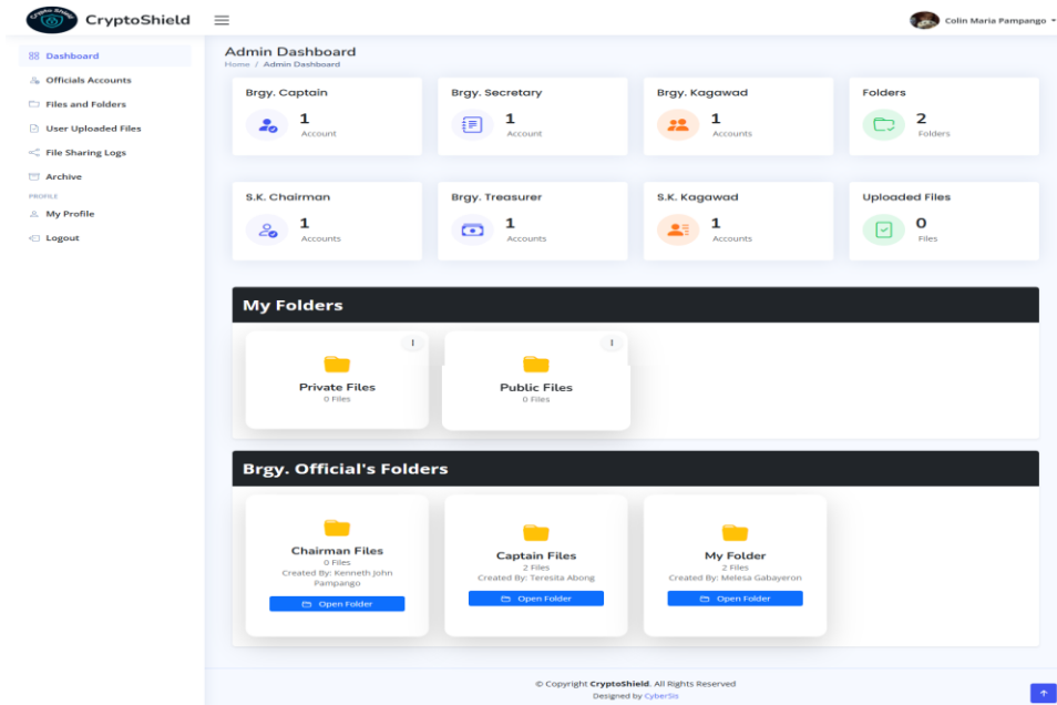
Figure 6. Admin Dashboard
