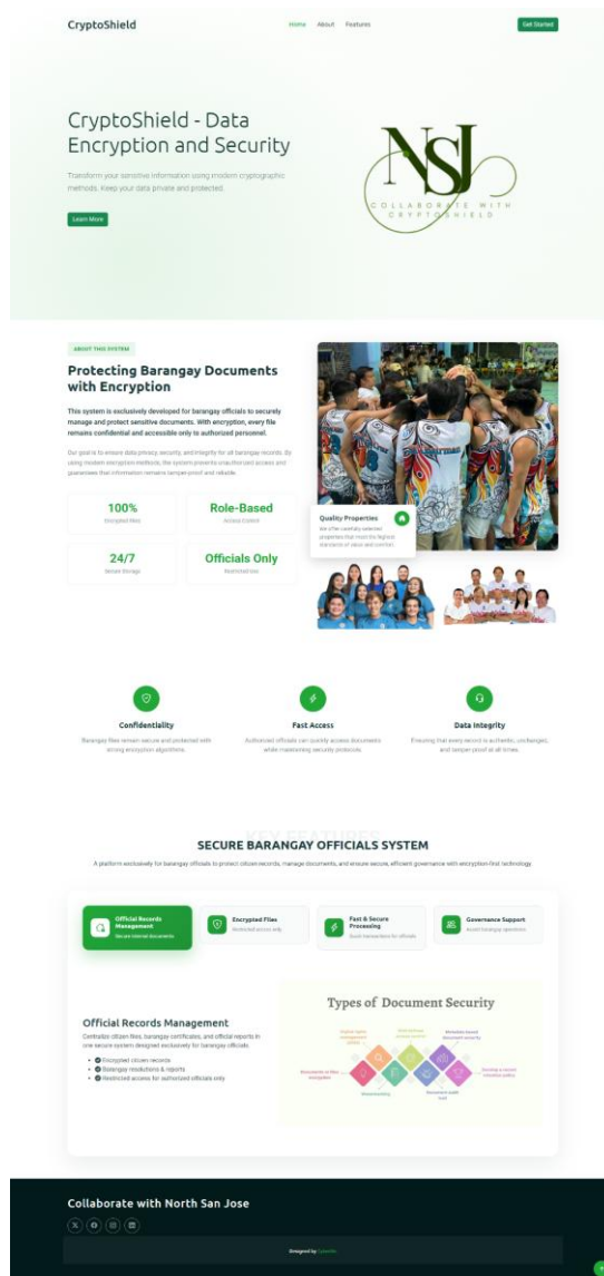
Figure 3. Landing Page
