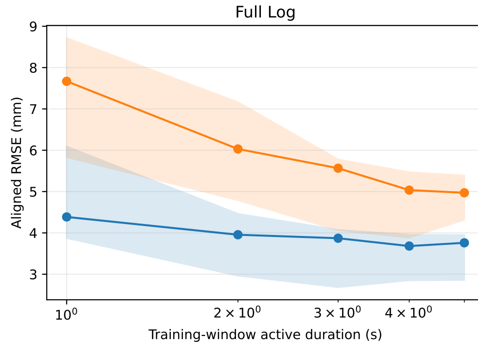
Mag-to-travel calibration learning curve
