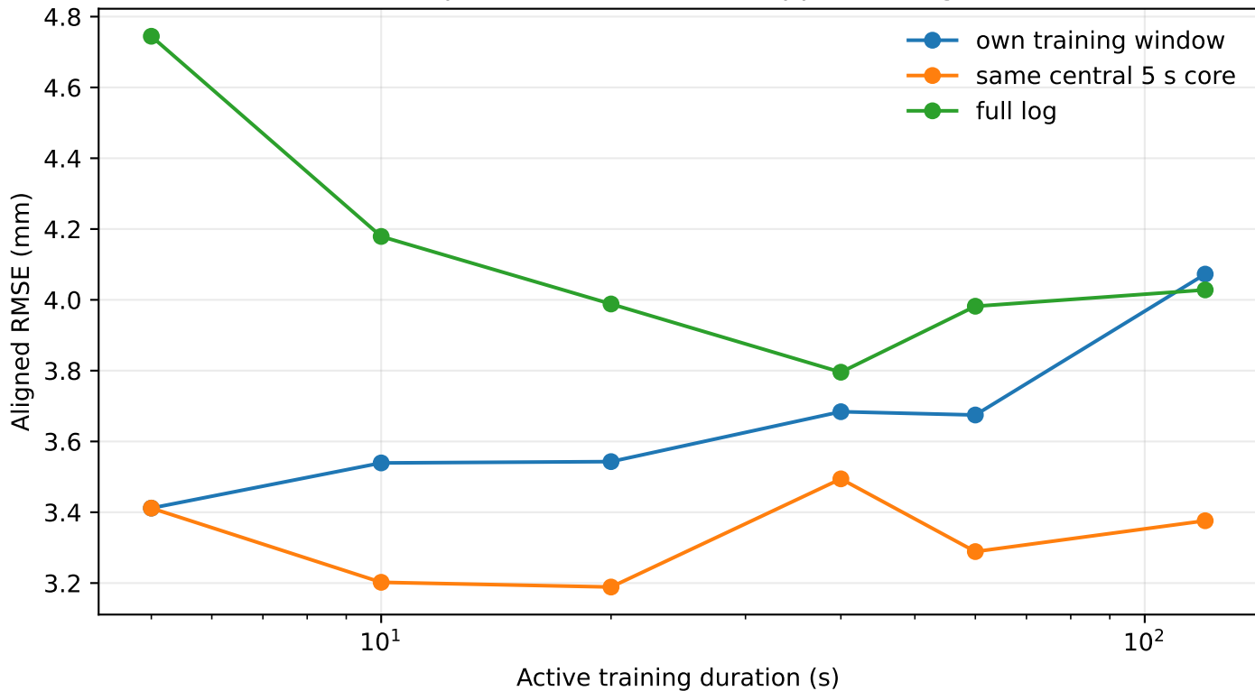
Front v1 self-supervised: evaluation support changes the trend
