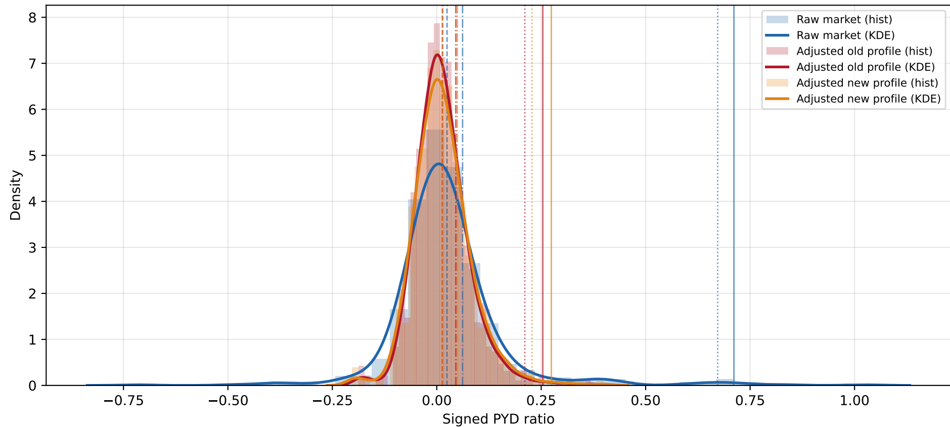
Distribution of signed PYD ratio Donor pool: FULL subset, n=685, adverse=376
