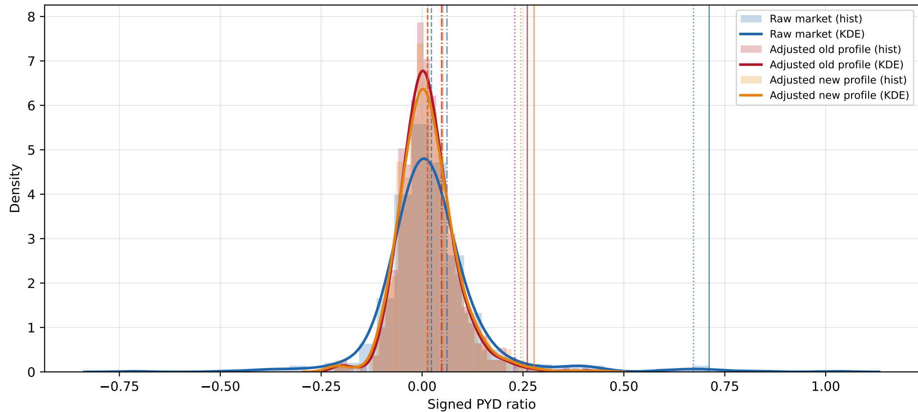
Distribution of signed PYD ratio Donor pool: FULL subset, n=695, adverse=379
