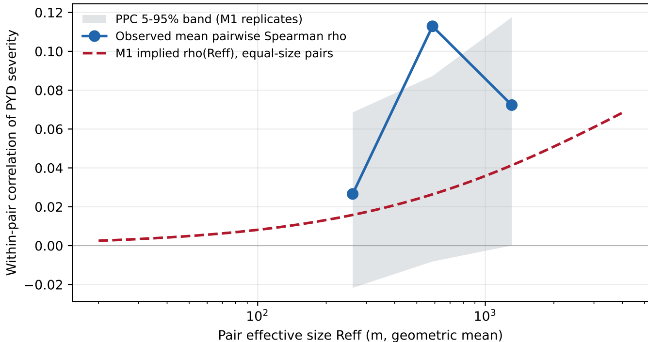
Correlation-vs-size profile: observed vs M1 posterior predictive
