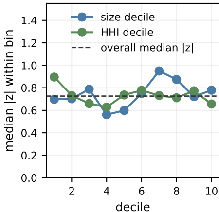
Median |z| is flat across size and HHI deciles
