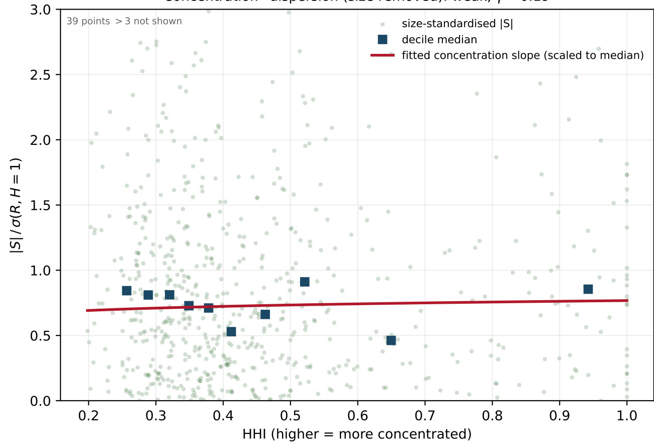
Concentration–dispersion (size removed): weak, \gamma = 0.19
