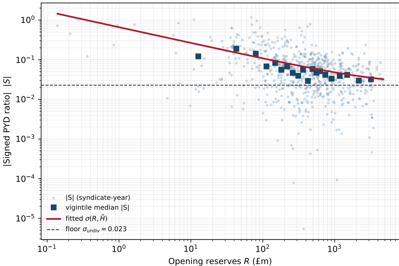
Size–dispersion: |S| decays with size toward the floor ( k = 0.60 )
