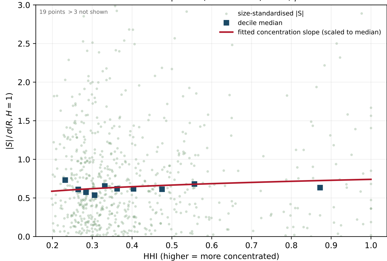
Concentration–dispersion (size removed): weak, \gamma = 0.48
