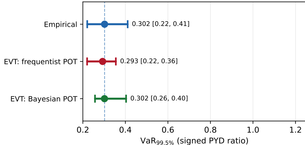
V2 (new profile) ( \hat{\xi} \approx 0.07 )
