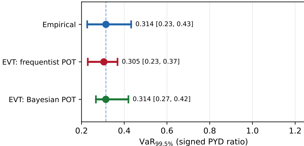
V1 (adjusted) ( \hat{\xi} \approx 0.07 )
