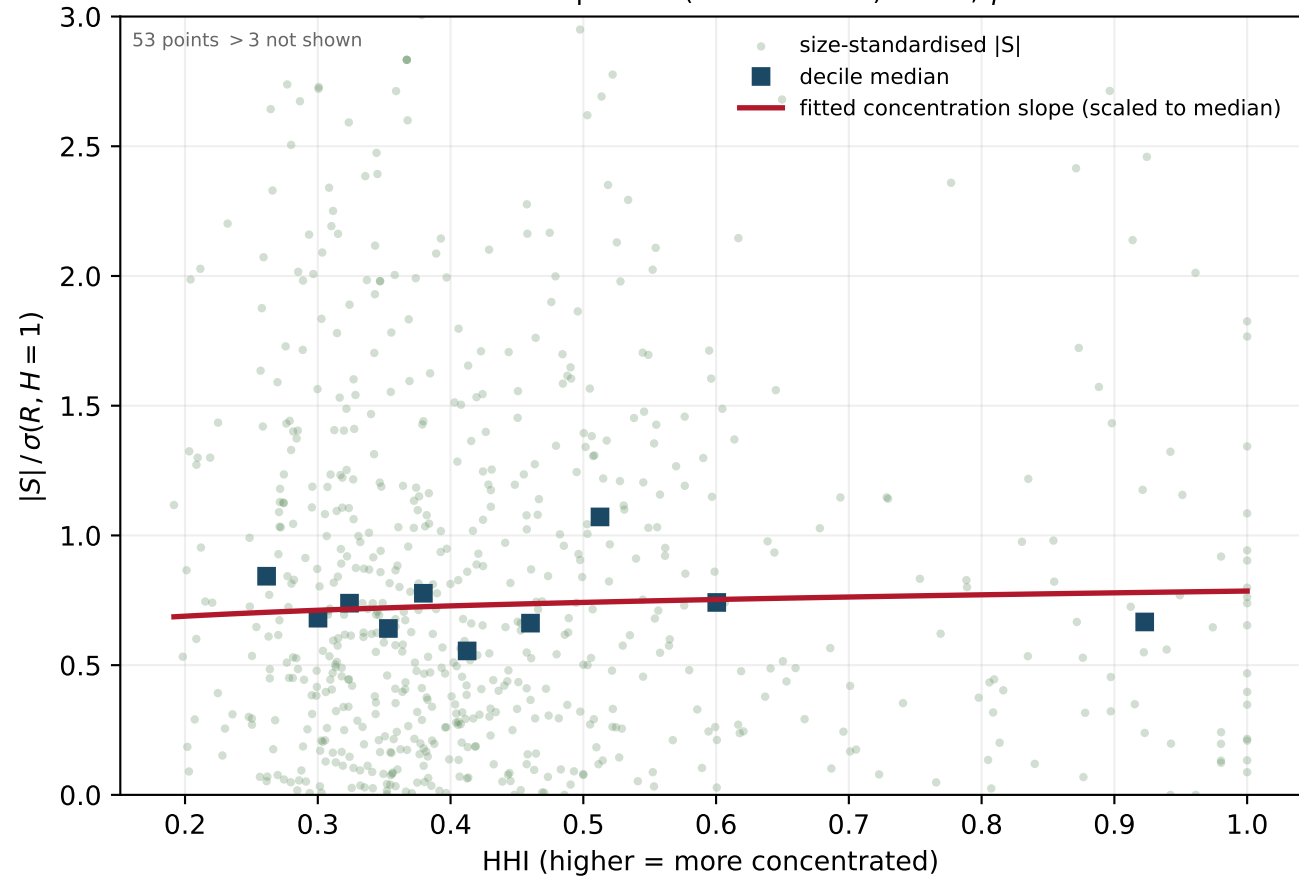
Concentration–dispersion (size removed): weak, \gamma = 0.24
