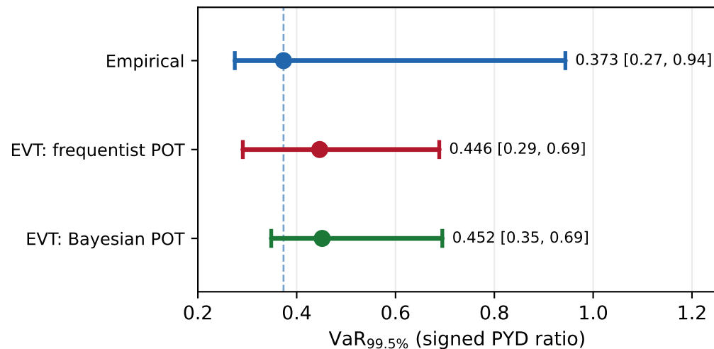
V2 (new profile) ( \hat{\xi} \approx 0.40 )
