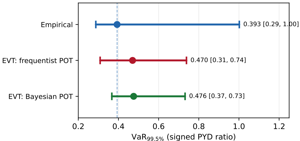
V1 (adjusted) ( \hat{\xi} \approx 0.40 )
