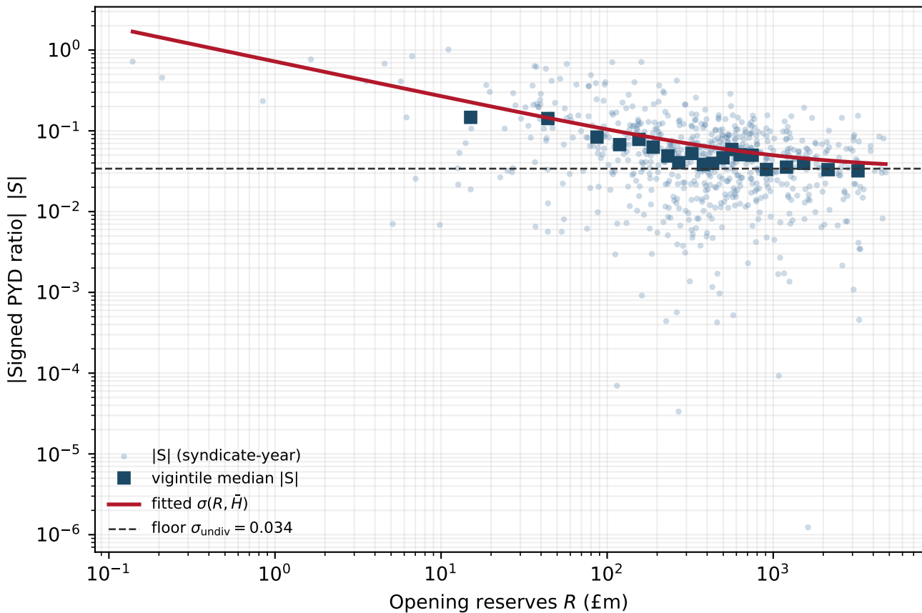
Size–dispersion: |S| decays with size toward the floor ( k = 0.57 )
