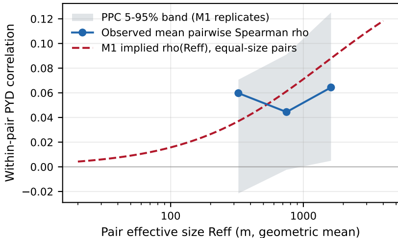
Correlation-vs-size profile: observed vs M1 posterior predictive
